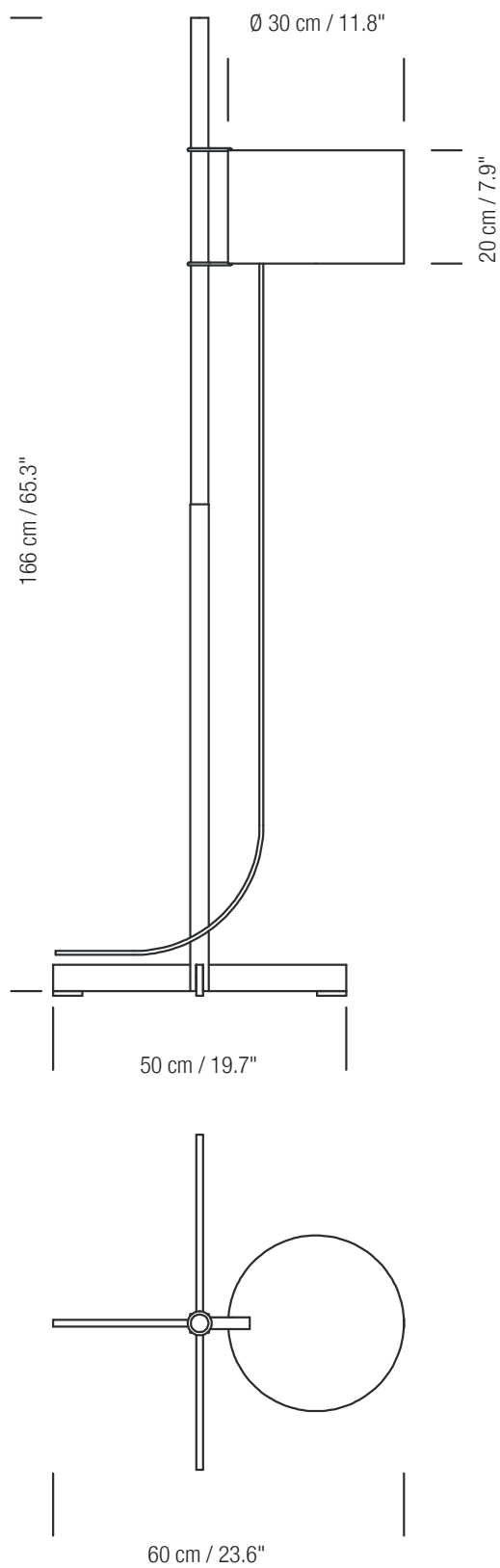
(1.)TMM table fixture
