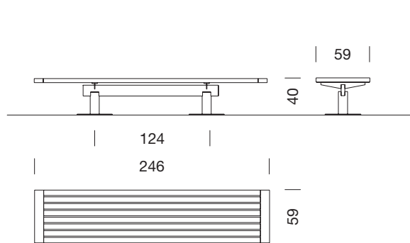
Nu bench 2,46 m without backrest
