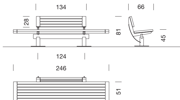
Nu bench 2,46 m with short backrest
