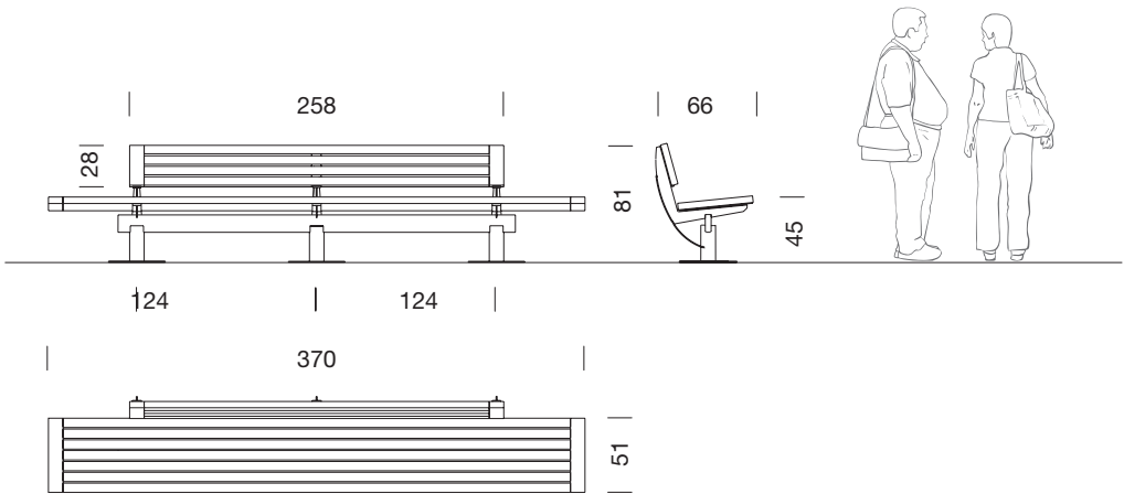
Nu bench 3,70m with backrest
