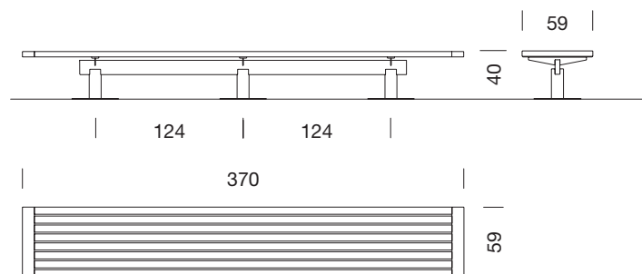
Nu bench 3,70 m without backrest
