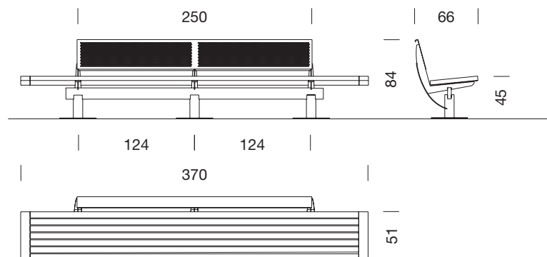
Nu bench 3,70m with metal backrest
