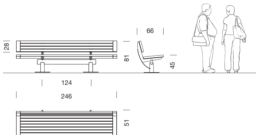
Nu bench 2,46 m with metal backrest
